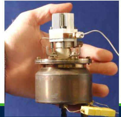
Ultra-Compact Hydrogen-Generator
