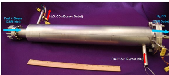
Fuel Reformer for Hydrogen Production
